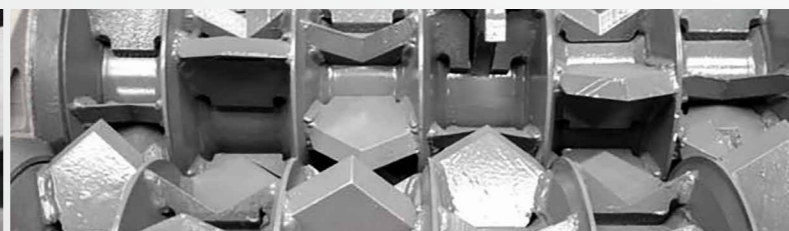
Shredding unit - triangular knives
